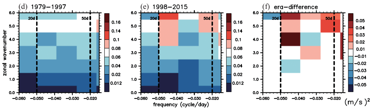
Fig. S1. Same as Fig. 2, but 250 hPa meridional wind (unit: \text{m s}^{-1} ). (d) - (f) are averaged by symmetric 10^\circ\text{S} - 10^\circ\text{N} .
