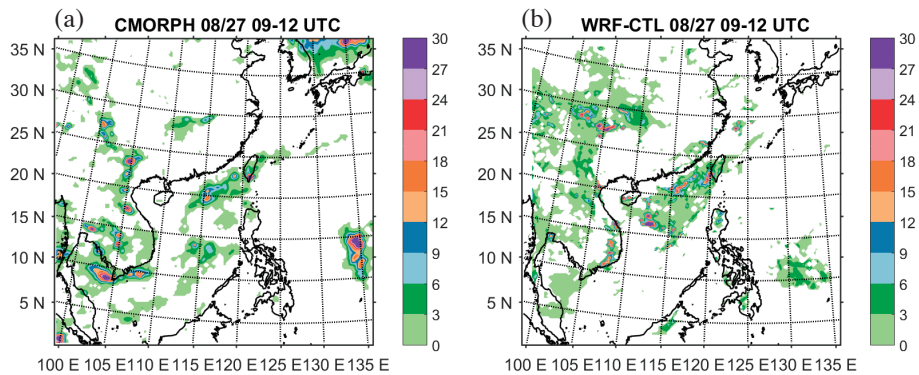
Fig. 4. The precipitation rate (unit: mm 3hr -1 ) from the (a) CMORPH satellite precipitation data and (b) 27-km CTL simulation at 09 - 12 UTC 27 August 2015.
