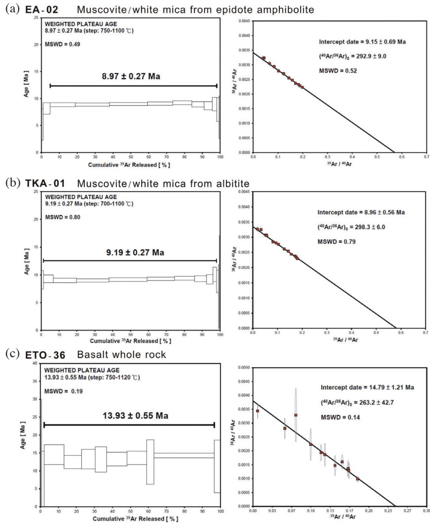
Fig. 5. 40 Ar/ 39 Ar age spectra and isotope correlation diagrams for samples (a) EA-02 white mica, (b) TKA-01 white mica, and (c) ETO-36 basalt whole rock.
