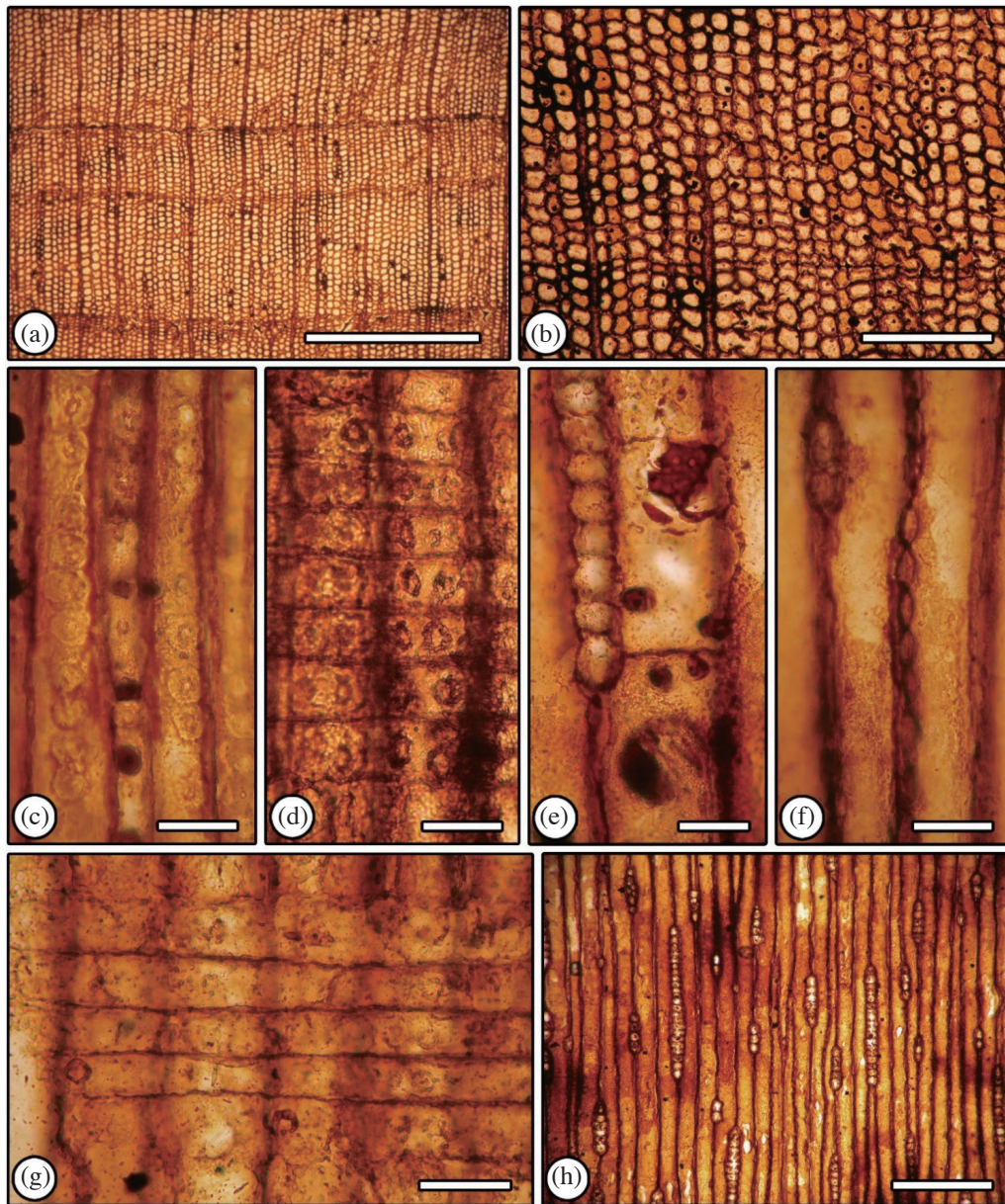
Fig. 2. Wood structure of Podocarpoxyton nageioides Y.-P. Lo and J.-M. Hu, sp. nov. (WL001). (a) Transverse section showing indistinct growth ring boundaries and abundant, diffuse axial parenchyma. Scale bar = 1 mm. (b) Transverse section showing the shape of tracheids, square to polygonal. Scale bar = 250 \mu\text{m} . (c) Radial section showing the intertracheary radial pitting uniseriate. Scale bar = 40 \mu\text{m} . (d) Radial section showing cupressoid to taxodioid cross-field pits. Scale bar = 25 \mu\text{m} . (e) Tangential section showing end walls of axial parenchyma smooth. Scale bar = 25 \mu\text{m} . (f) Tangential section showing intertracheary radial pits and torus. Scale bar = 40 \mu\text{m} . (g) Radial section showing end and horizontal walls of ray parenchyma smooth and thin. Scale bar = 40 \mu\text{m} . (h) Tangential section showing ray parenchyma uniseriate and cells height. Scale bar = 250 \mu\text{m} .
