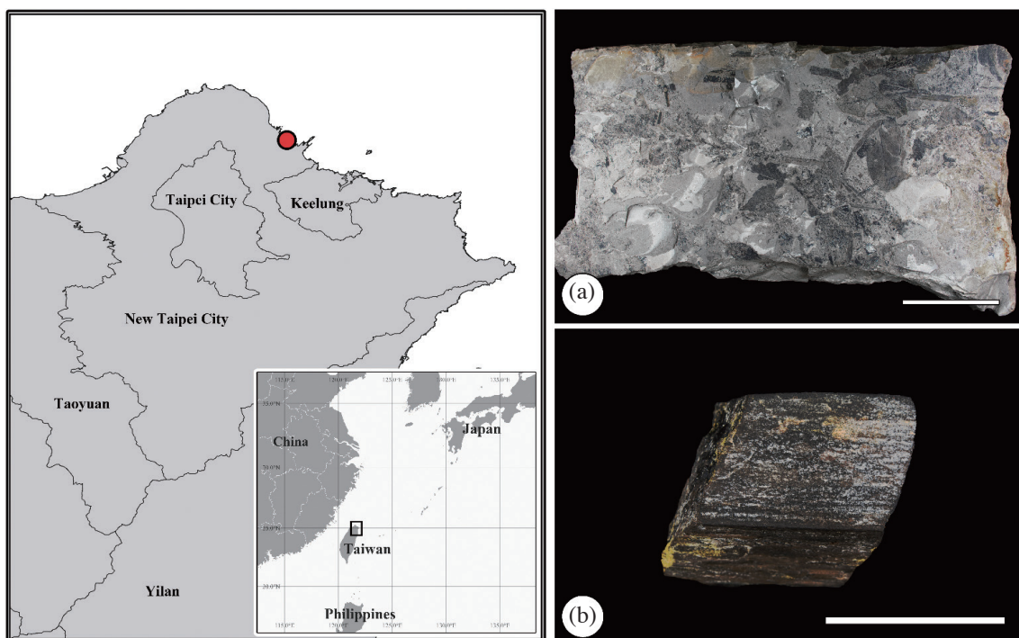
Fig. 1. The sampling locality (red spot) is in Wanli distinct, Northern Taiwan. (a) Leaf fossils from the same locality. Scale bar = 10 cm. (b) The fossil wood sample of this article (WL001). Scale bar = 5 cm.
