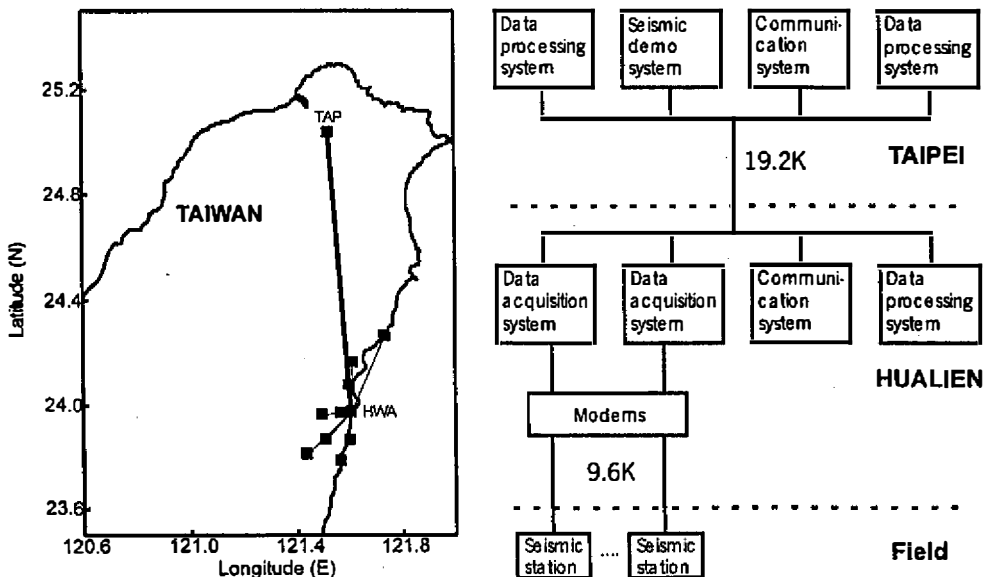
Fig. 2. The prototype earthquake early warning system in Hualien (Plan A). This system consists of 10 three-component accelerometers telemetered digitally via 9600-baud telephone lines to the CWB Hualien Station. At the Hualien Station, the incoming digital signals are processed in real time and the results are telemetered to the CWB Headquarters in Taipei.
