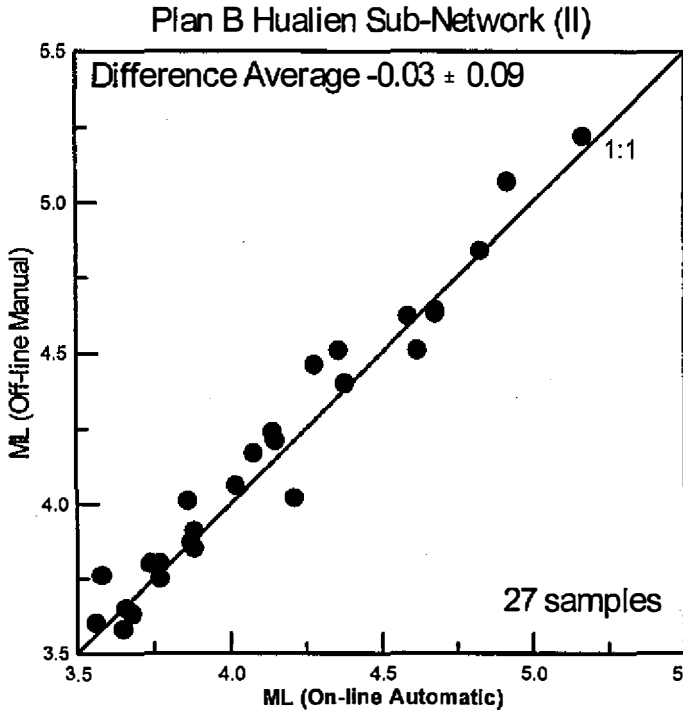
Fig. 9. Relationship between the automatic-determined magnitude and the manual-determined magnitude for twenty-seven events recorded by the Plan B Hualien sub-network (II).
