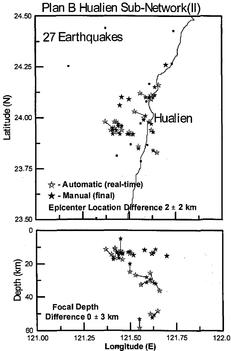
Fig. 8. Comparison of the automatic location and the manual location determined by the Plan B Hualien sub-network (II). The small solid squares are present the station location of this network.
