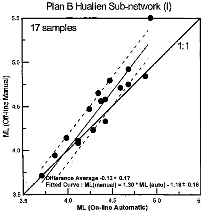
Fig. 6. Relationship between the automatic-determined magnitude and the manual-determined magnitude for seventeen events recorded by the Plan B Hualien sub-network (I). The on-line determined magnitudes are smaller than the off-line values, especially for earthquake magnitude larger than 4.25.
