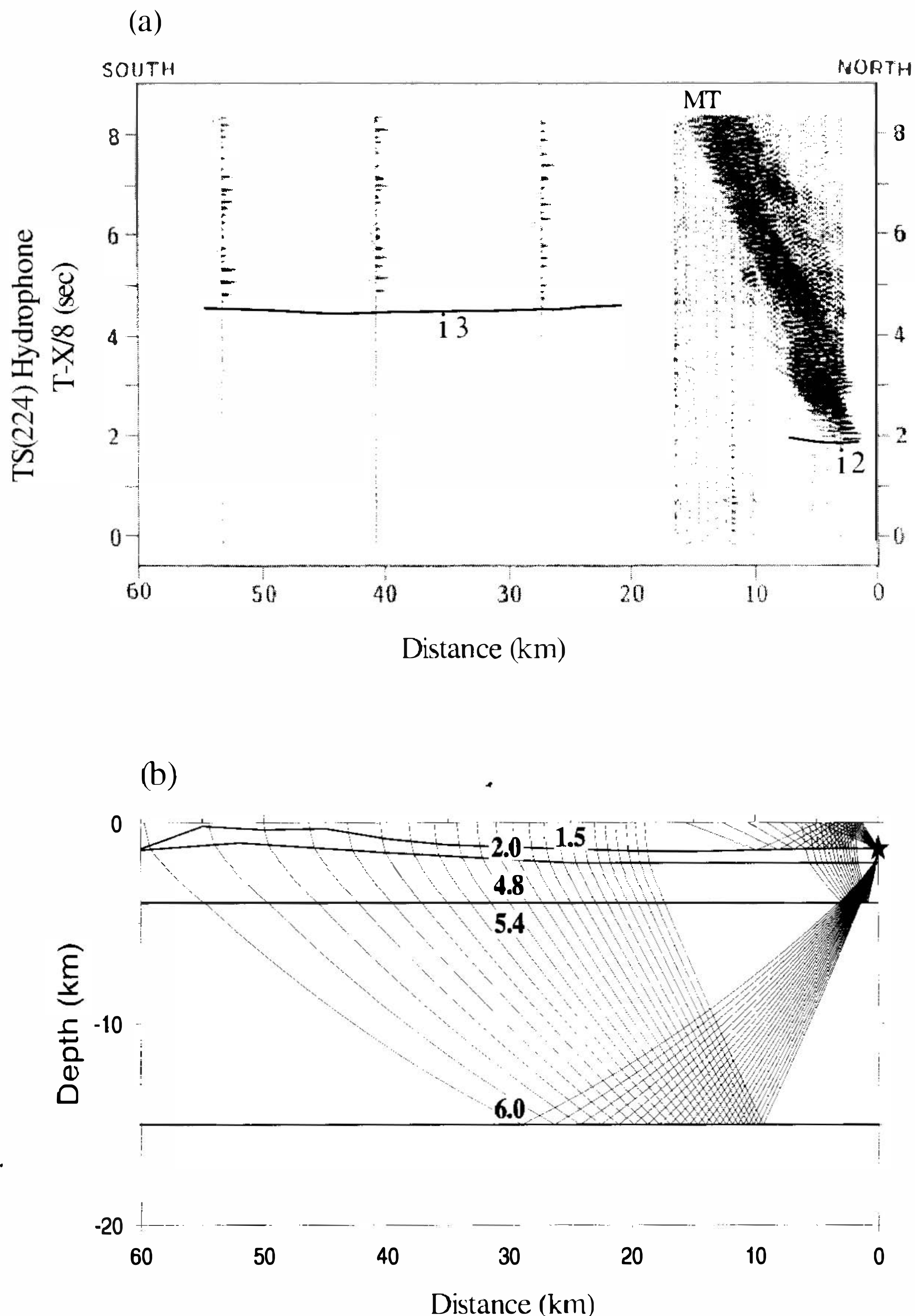
Fig. 10. (a) Observed seismograms and predicted travel time curves of profile L85-2. The phase, i3, in an offset range of 27-54 km is interpreted as reflected waves from a lower intercrustal layer (PiP phase). The MT phases are explained as multiples. (b) Velocity structure and ray diagram, with the vertical exaggeration taken as 1.6:1.
