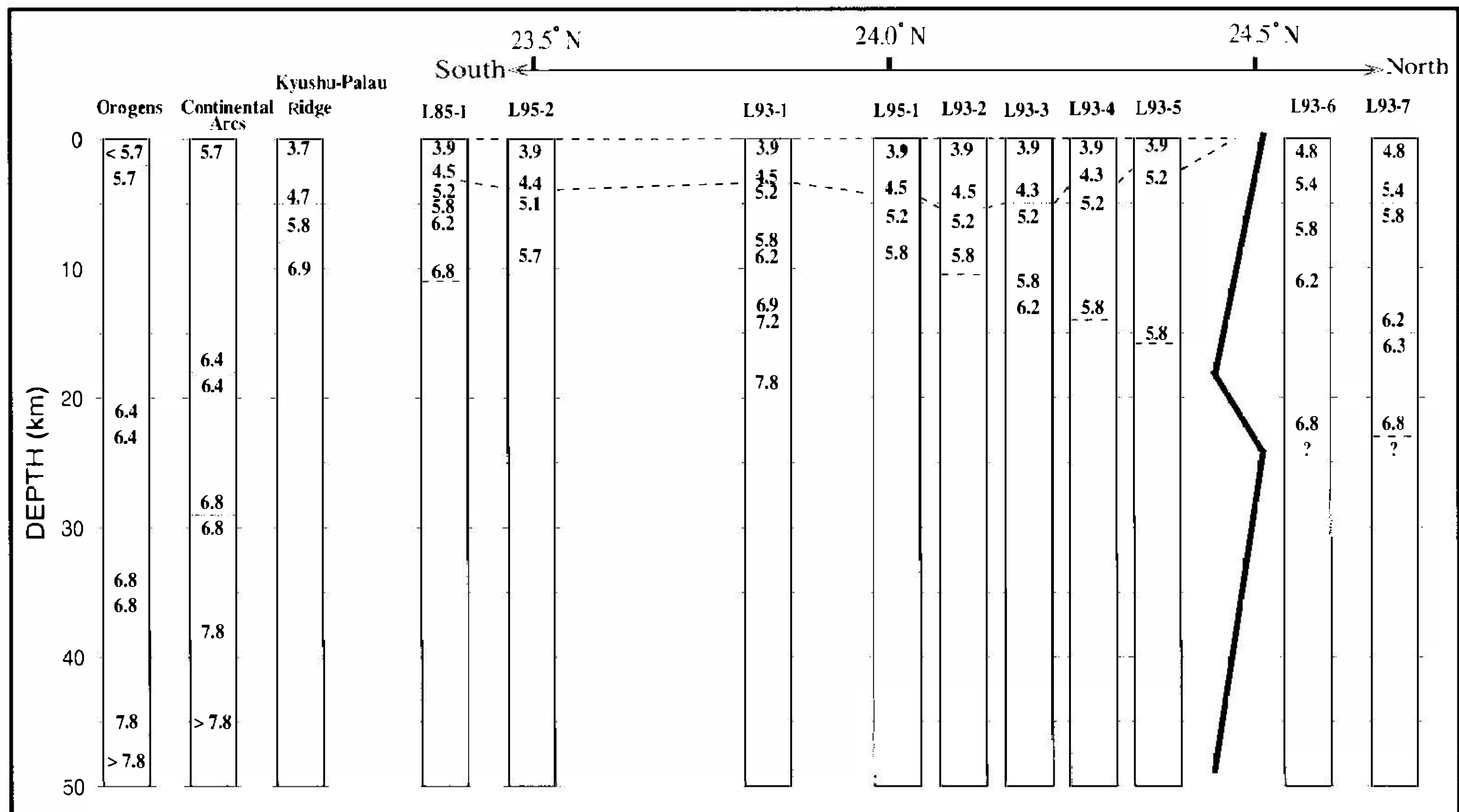
Fig. 11. Comparison between the average crustal velocity structures of orogens, continental arcs and the Kyushu-Palau Ridge (the three on the left) and the velocity models to the west (a) and east (b) of the LV fault constructed in this study (without water and sedimentary layer). The shaded parts show the distribution of the velocity structure ranging from about 5.7 km/s to 6.4 km/s. See text for explanation.
