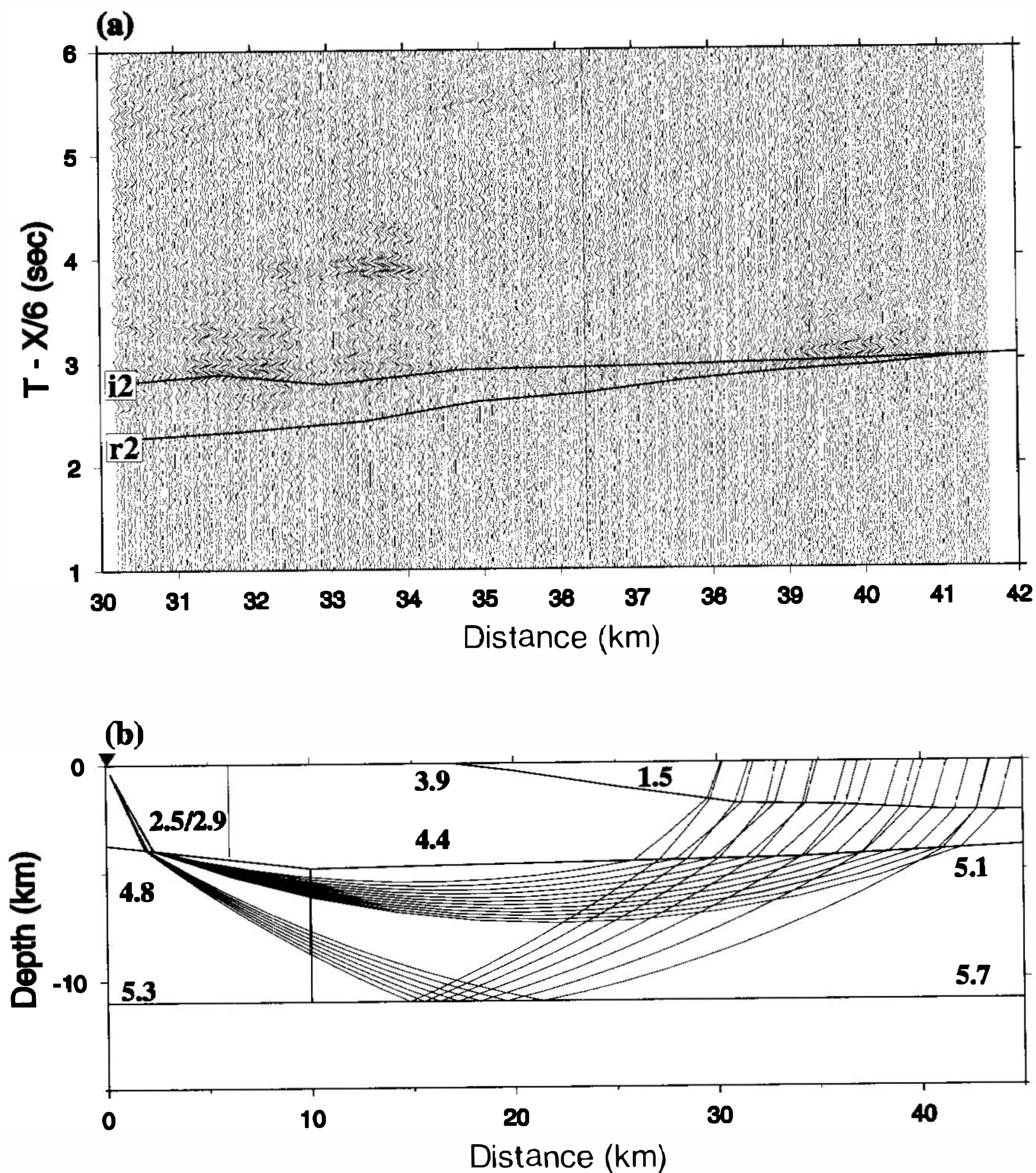
Fig. 8. (a) Observed seismograms recorded by the EHY station and calculated travel time curves along profile L95-2. The i2 and r2 phases are explained as reflected and refracted waves. (b) Velocity structure and ray diagram, with the vertical exaggeration taken as 1:1.
