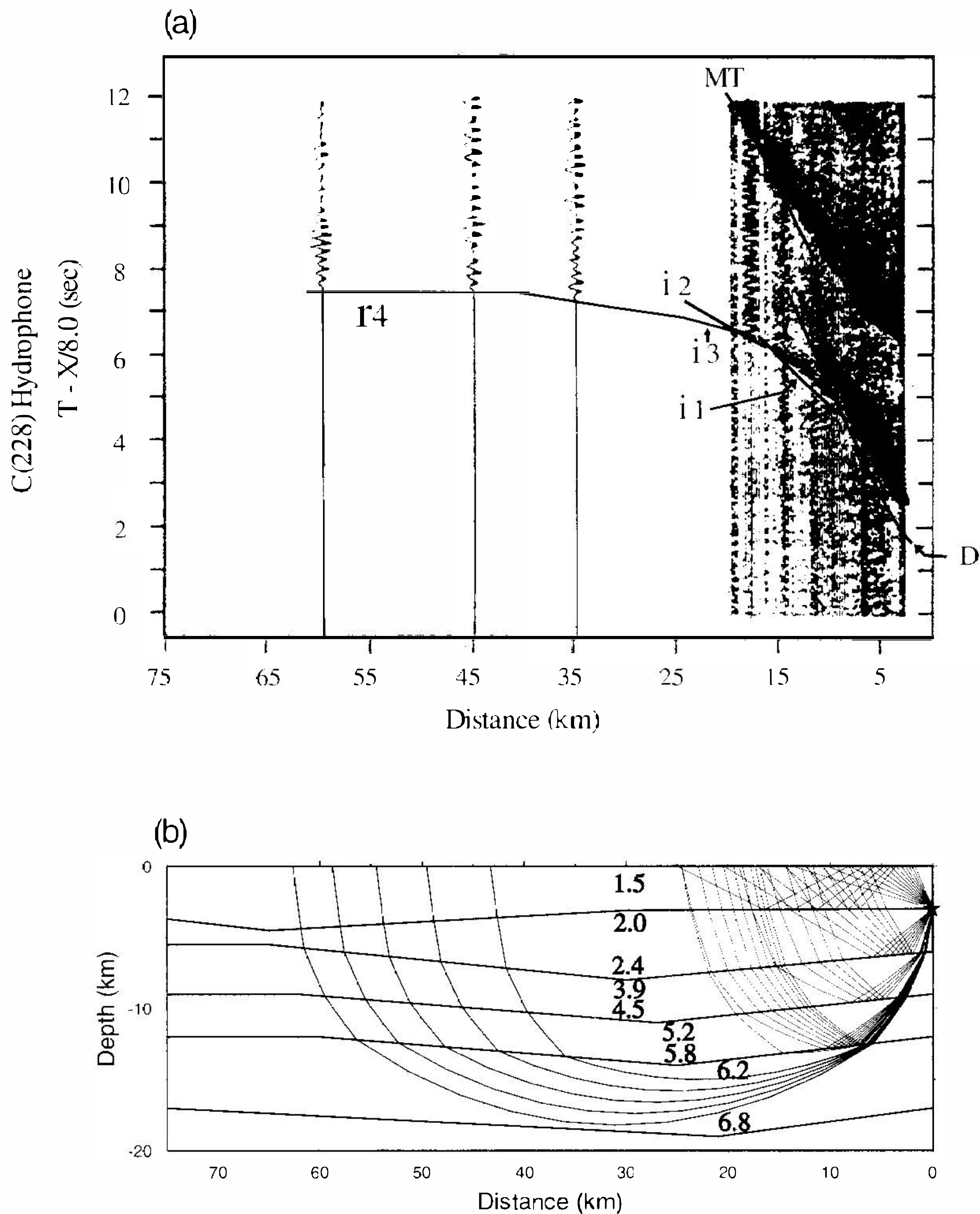
Fig. 9. (a) Observed seismograms recorded by the OBS-C and predicted travel time curves along profile L85-1. The D and MT phases are explained as directed waves and multiples, respectively. (b) Velocity structure and ray diagram, with the vertical exaggeration taken as 1.4:1.
