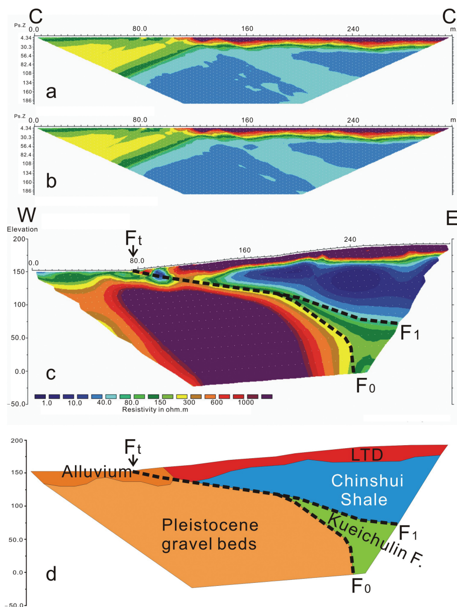
Fig. 5. Measured data and interpreted results of Profile C-C'. (a) Measured apparent resistivity pseudosection; (b) Calculated apparent resistivity pseudosection; (c) Interpretative model; and (d) Geological section deduced from (c). F_t : terrace scarp; F_1 : Houli fault; and F_0 : Sanyi fault.
