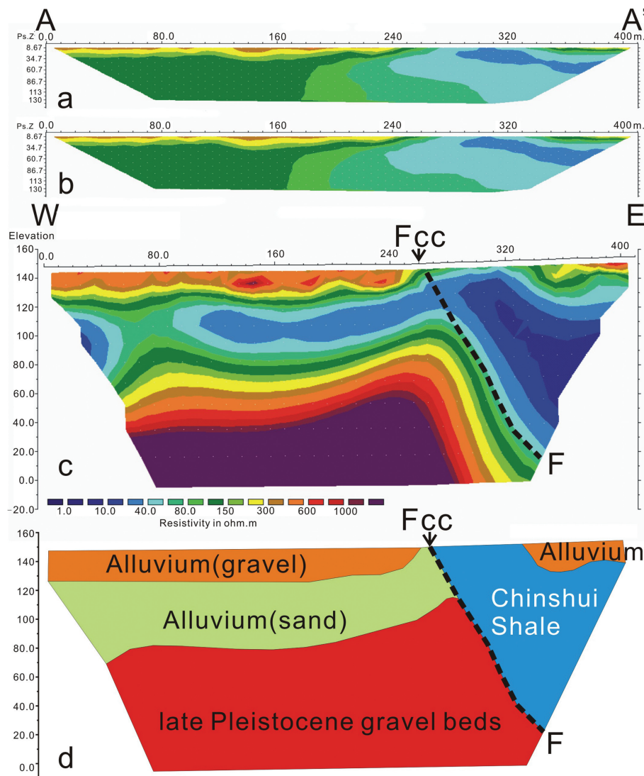
Fig. 3. Measured data and interpreted results of Profile A-A'. (a) Measured apparent resistivity pseudosection; (b) Calculated apparent resistivity pseudosection; (c) Interpretative model; and (d) Geological section deduced from (c). F_{cc} : surface rupture induced by the 1999 Chi-Chi earthquake. F: the main fault zone of the Chelungpu fault system in which the Chi-Chi earthquake rupture is involved, where the Chinshui Shale thrusts on the alluvium and the late Pleistocene gravel beds.
