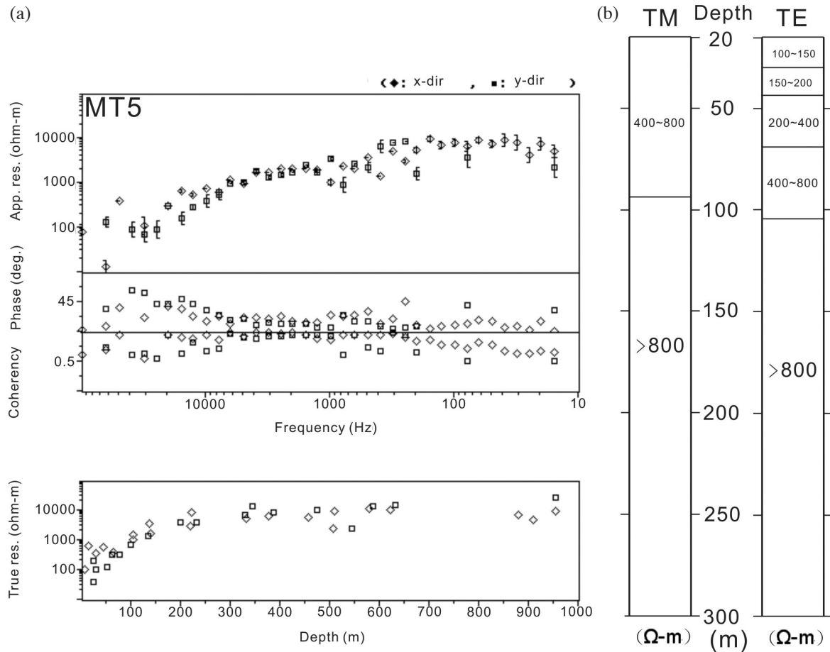
Fig. 10. (a) The MT sounding results of MT5; and (b) Resistivity columns of MT5 interpreted from the data of TE and TM modes.
