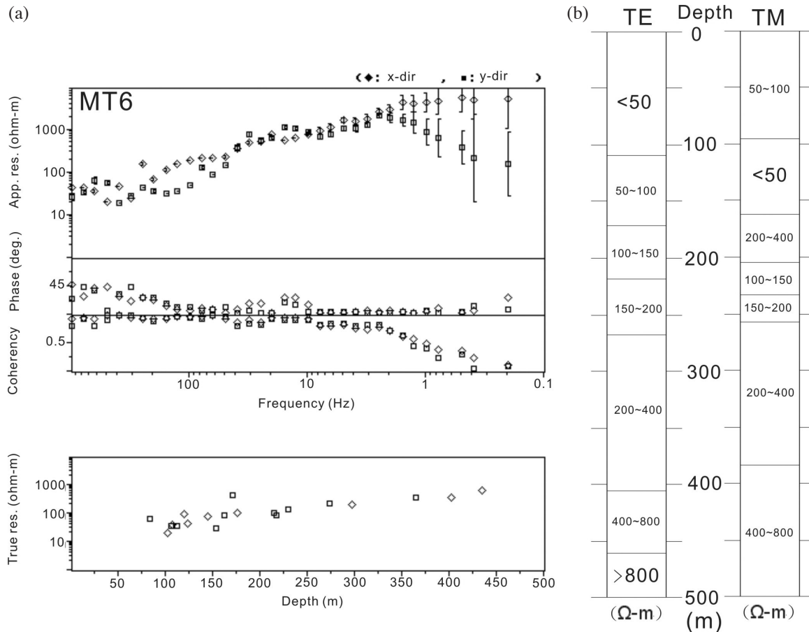
Fig. 11. (a) The MT sounding results of MT6; and (b) The resistivity columns of MT6 interpreted from the data of TE and TM modes.
