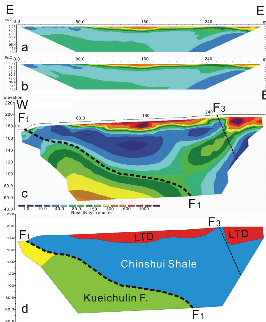
Fig. 7. Measured data and interpreted results of Profile E-E'. (a) Measured apparent resistivity pseudosection; (b) Calculated apparent resistivity pseudosection; (c) Interpretative model; and (d) Geological section deduced from (c). F_t : terrace scarp; F_1 : the main shear zone of the Chelungpu fault system (Houli fault) where the uppermost part of the Chinshui Formation thrusts on the Alluvium; and F_3 : minor fault.
