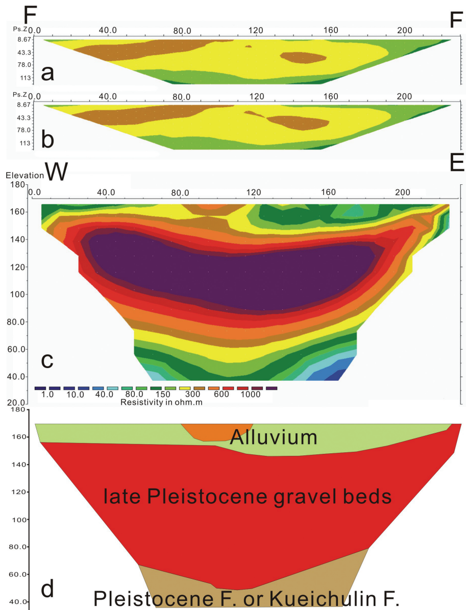
Fig. 8. Measured data and interpreted results of Profile F-F'. (a) Measured apparent resistivity pseudosection; (b) Calculated apparent resistivity pseudosection; (c) Interpretative model; and (d) Geological section deduced from (c).
