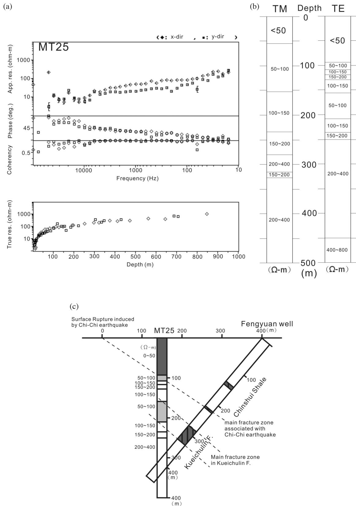
Fig. 9. (a) The MT sounding results of MT25; (b) Resistivity columns of MT25 interpreted from the data of TE and TM modes; and (c) The resistivity column of TE mode and the rock formations recognized from the cores of the Fengyuan well.
