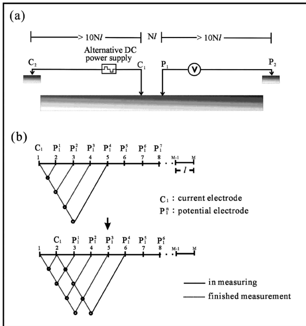
Fig. 2. Electrode configuration of the pole-pole array used in RIP. (a) The sounding electrodes C_1 and P_1 are arranged on the surface of the profile to be investigated. They have a electrode-spacing varying from l to Nl . The remote electrodes C_2 and P_2 are fixed at distance from the profile. (b) A number of electrodes are arranged on the surface of the profile to enable the automatic changing of the sounding electrodes.
