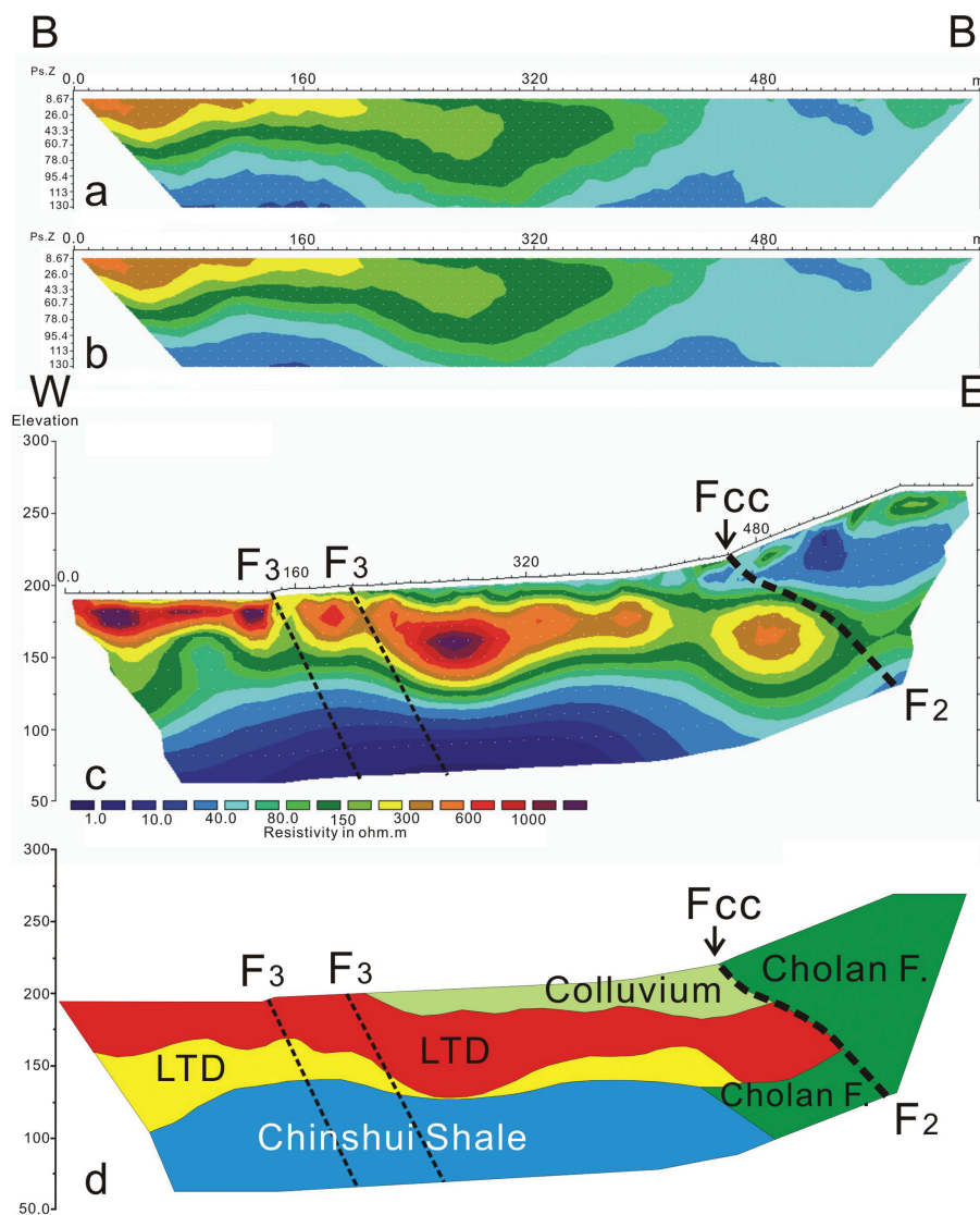
Fig. 4. Measured data and interpreted results of Profile B-B'. (a) Measured apparent resistivity pseudosection; (b) Calculated apparent resistivity pseudosection; (c) Interpretative model; and (d) Geological section deduced from (c). F_{cc} : surface rupture induced by the 1999 Chi-Chi earthquake; F_2 : subsurface rupture associated with the Chi-Chi earthquake; LTD: the lateritic terrace deposits; and F_3 : minor fault.
