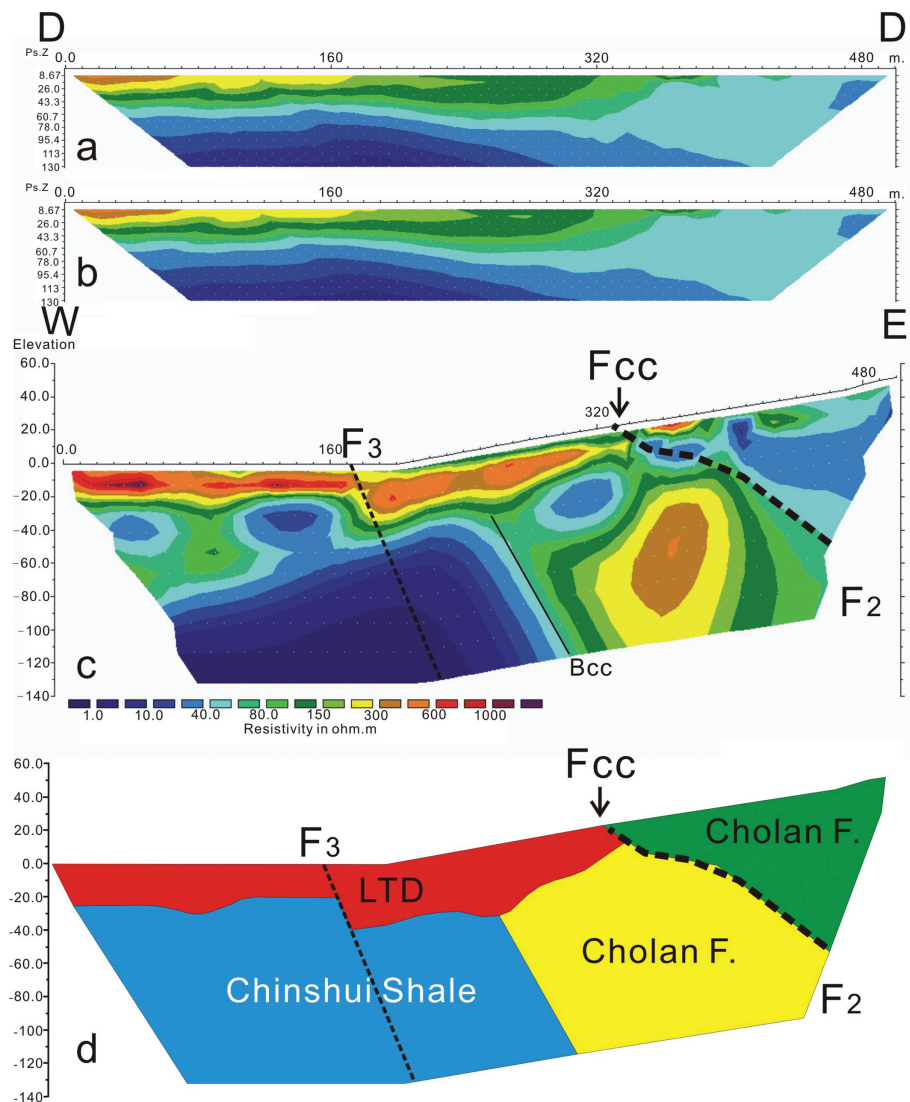
Fig. 6. Measured data and interpreted results of Profile D-D'. (a) Measured apparent resistivity pseudosection; (b) Calculated apparent resistivity pseudosection; (c) Interpretative model; and (d) Geological section deduced from (c). F_{cc} : surface rupture induced by the 1999 Chi-Chi earthquake; F_2 : Chi-Chi earthquake rupture [it developed in the Cholan Formation, the uppermost part of the Cholan Formation overlies the lateritic terrace deposits (LTD)]; and F_3 : minor fault.
