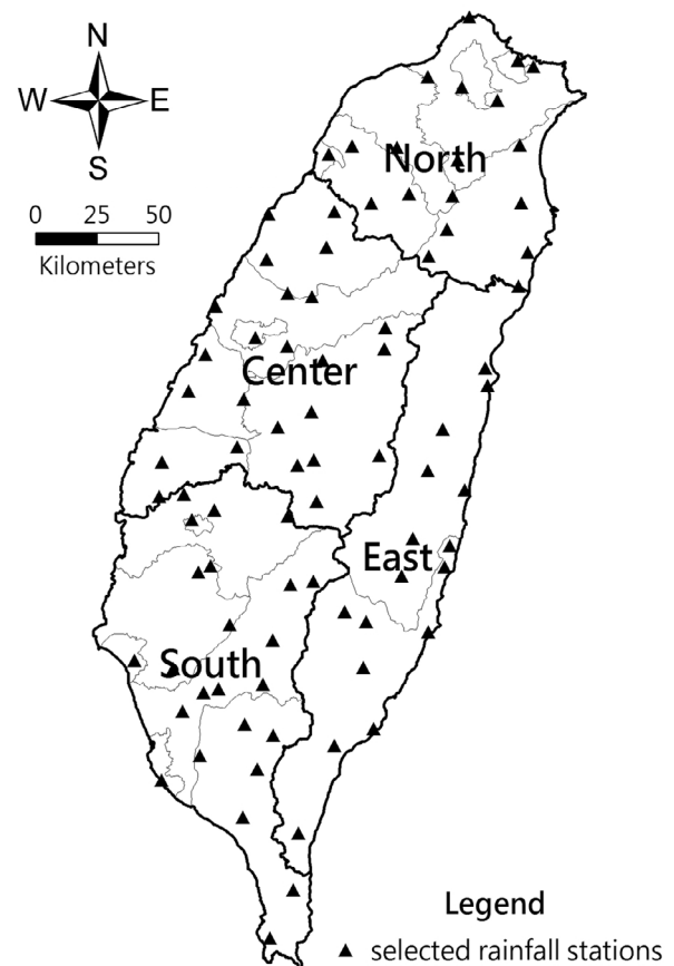
Fig. 1. Distribution and locations of four water resources regions and 83 rainfall stations.
