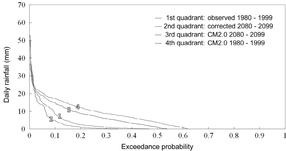
Fig. 4. Exceedance distribution of each quadrant in January of Taipei.
