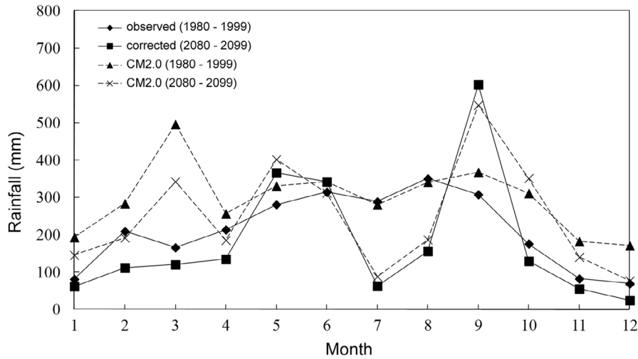
Fig. 2. Comparison of observations and adjusted CM2.0 projections in Taipei.
