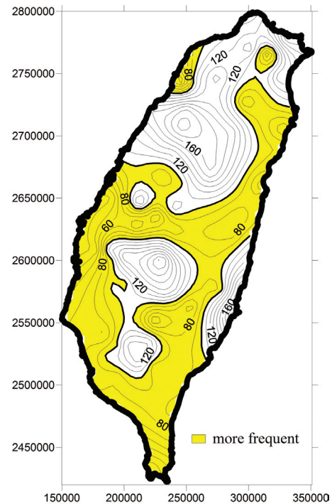
Fig. 12. Future return period of maximum 3-day rainfall (2080 - 2099) with an intensity of today's 100-yr events (1980 - 1999).
