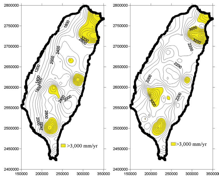
Fig. 5. Comparison of annual rainfall in Taiwan between 1980 - 1999 (L) and 2080 - 2099 (R), under A1B scenario and based on an ensemble of 5 climate models.
