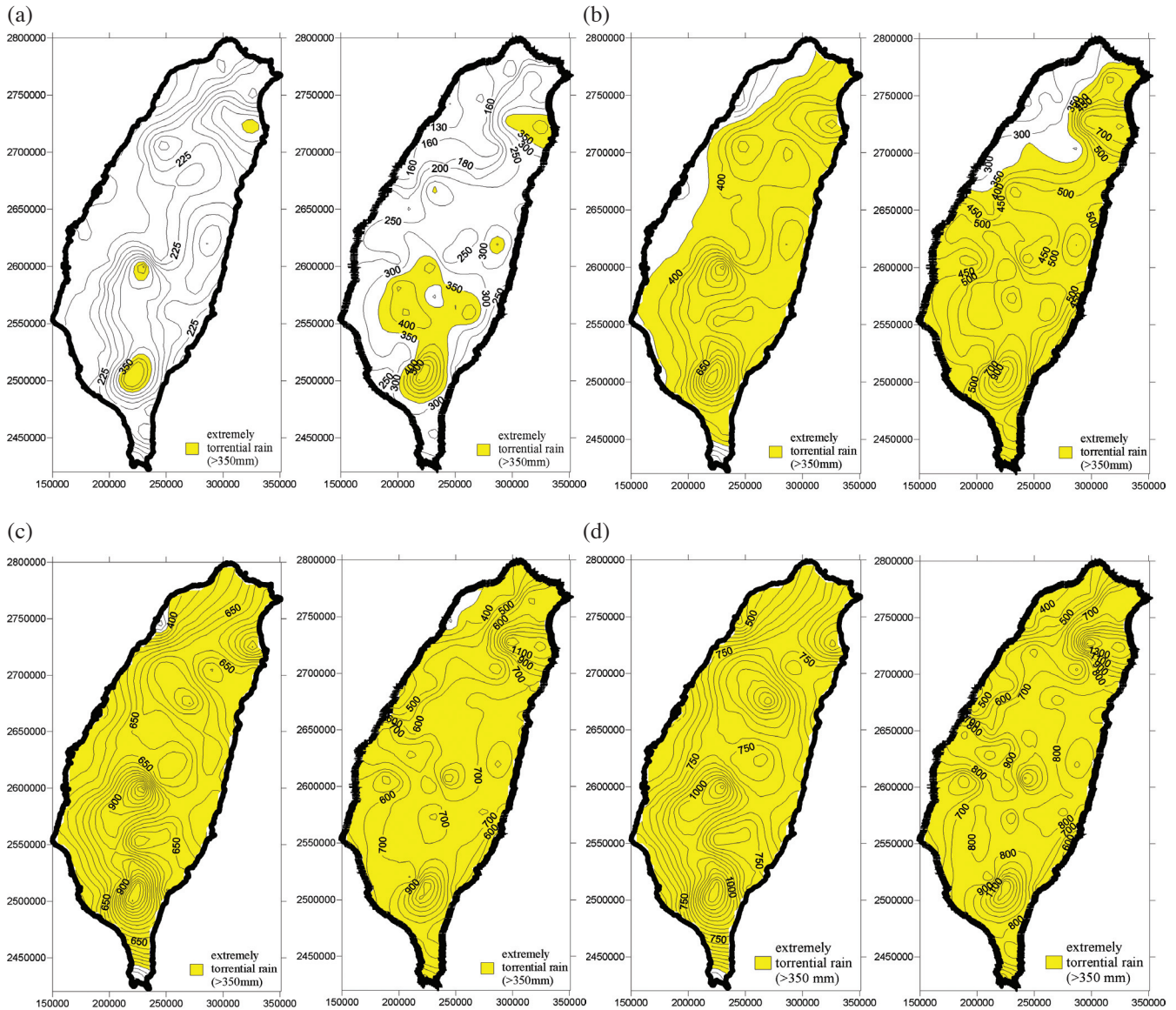
Fig. 9. (a) Comparison of 2-yr maximum 1-day rainfall in Taiwan between 1980 - 1999 (L) and 2080 - 2099 (R), under A1B scenario and based on an ensemble of 5 climate models. (b) Comparison of 10-yr maximum 1-day rainfall in Taiwan between 1980 - 1999 (L) and 2080 - 2099 (R), under A1B scenario and based on an ensemble of 5 climate models. (c) Comparison of 50-yr maximum 1-day rainfall in Taiwan between 1980 - 1999 (L) and 2080 - 2099 (R), under A1B scenario and based on an ensemble of 5 climate models. (d) Comparison of 100-yr maximum 1-day rainfall in Taiwan between 1980 - 1999 (L) and 2080 - 2099 (R), under A1B scenario and based on an ensemble of 5 climate models.
