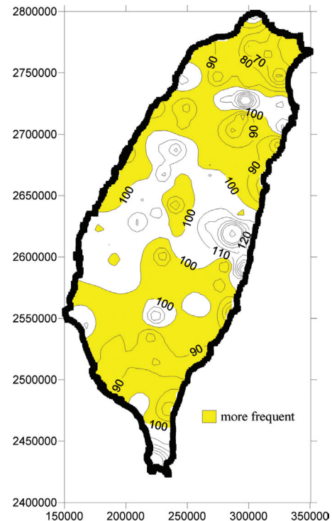
Fig. 8. Future return period of maximum consecutive dry days (2080 - 2099) with an intensity of today's 100-yr events (1980 - 1999).
