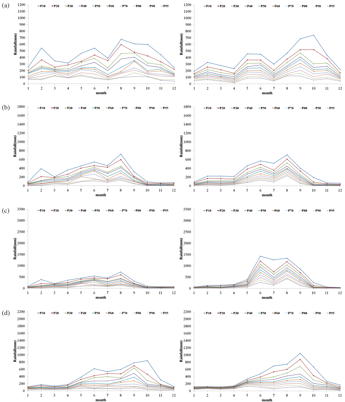
Fig. 6. (a) Comparison of exceedance curves of monthly rainfall in northern Taiwan between 1980 - 1999 (L) and 2080 - 2099 (R), under A1B scenario and based on an ensemble of 5 climate models. (b) Comparison of exceedance curves of monthly rainfall in central Taiwan between 1980 - 1999 (L) and 2080 - 2099 (R), under A1B scenario and based on an ensemble of 5 climate models. (c) Comparison of exceedance curves of monthly rainfall in southern Taiwan between 1980 - 1999 (L) and 2080 - 2099 (R), under A1B scenario and based on an ensemble of 5 climate models. (d) Comparison of exceedance curves of monthly rainfall in eastern Taiwan between 1980 - 1999 (L) and 2080 - 2099 (R), under A1B scenario and based on an ensemble of 5 climate models.
