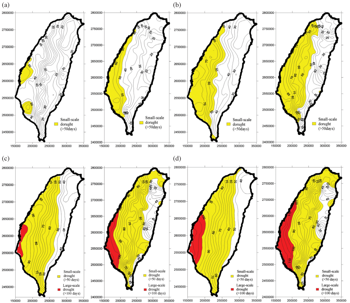
Fig. 7. (a) Comparison of 2-yr maximum consecutive dry days in Taiwan between 1980 - 1999 (L) and 2080 - 2099 (R), under A1B scenario and based on an ensemble of 5 climate models. (b) Comparison of 10-yr maximum consecutive dry days in Taiwan between 1980 - 1999 (L) and 2080 - 2099 (R), under A1B scenario and based on an ensemble of 5 climate models. (c) Comparison of 50-yr maximum consecutive dry days in Taiwan between 1980 - 1999 (L) and 2080 - 2099 (R), under A1B scenario and based on an ensemble of 5 climate models. (d) Comparison of 100-yr maximum consecutive dry days in Taiwan between 1980 - 1999 (L) and 2080 - 2099 (R), under A1B scenario and based on an ensemble of 5 climate models.
