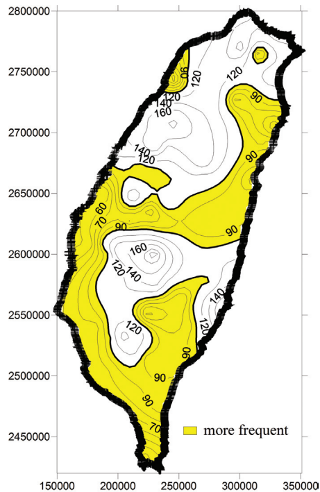
Fig. 11. Future return period of maximum 2-day rainfall (2080 - 2099) with an intensity of today's 100-yr events (1980 - 1999).
