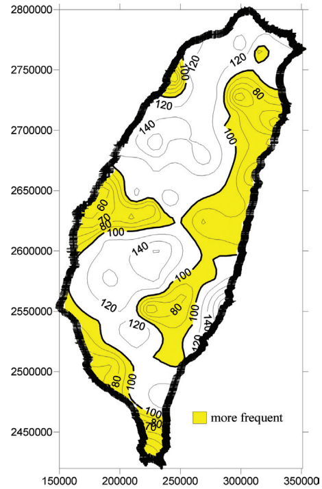
Fig. 10. Future return period of maximum 1-day rainfall (2080 - 2099) with an intensity of today’s 100-yr events (1980 - 1999).
