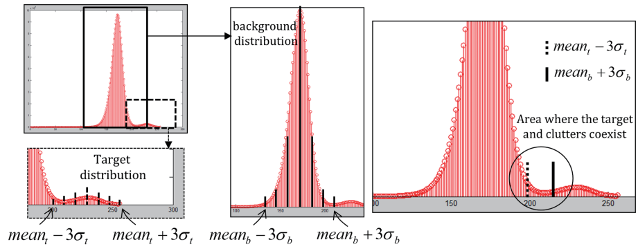
Fig. 5. Ranges of intensity for targets and background clutter. (Color online only)
