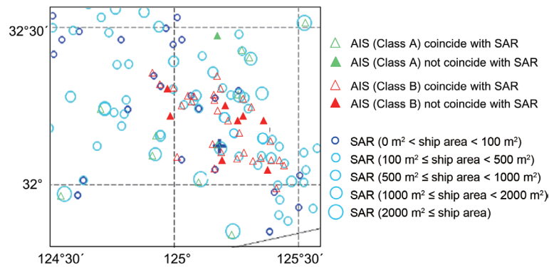
Fig. 10. Comparison of ships detected by our method and those collected by AIS. (Color online only)
