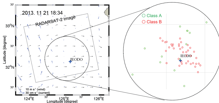
Fig. 2. Wind and water current speeds in the test area at RADARSAT-2 Wide Beam Mode data acquisition time, and the data coverage (left) and ship information collected by AIS (right). (Color online only)
