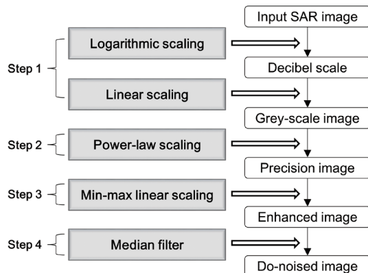
Fig. 3. Procedure for proposed automatic SAR image enhancement.
