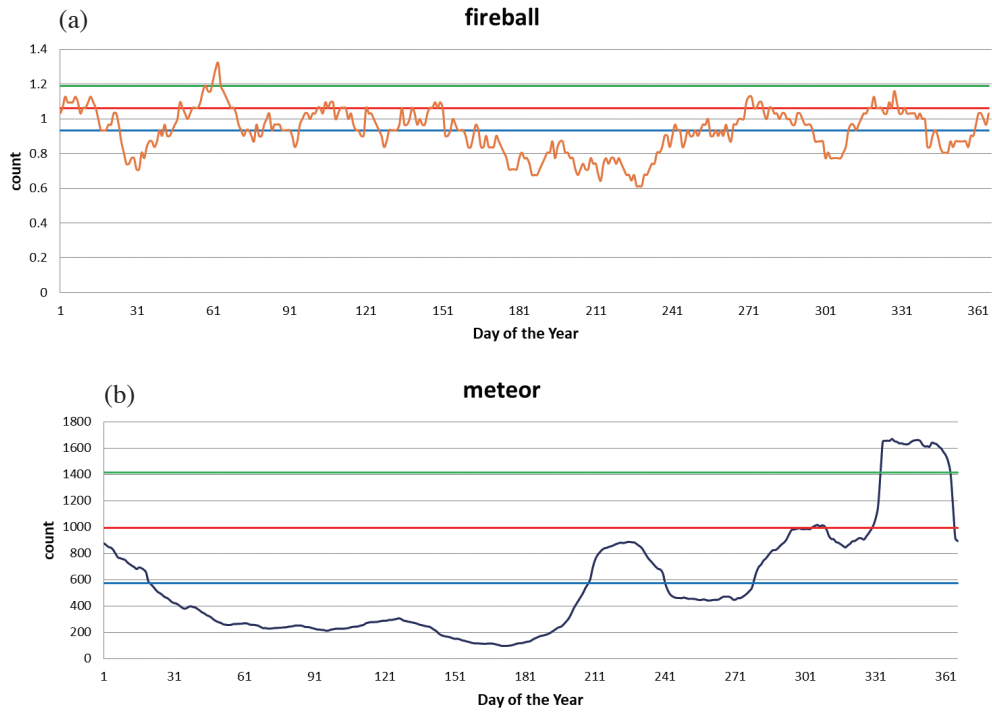
Fig. 4. (a) The graph of fireballs with their moving average. The blue line is the average daily occurrence frequency, and the red and green lines are 1\sigma and 2\sigma level. (b) The graph of meteors with their moving average. The blue line is the average daily occurrence frequency, and the red and green lines are 1\sigma and 2\sigma level.
