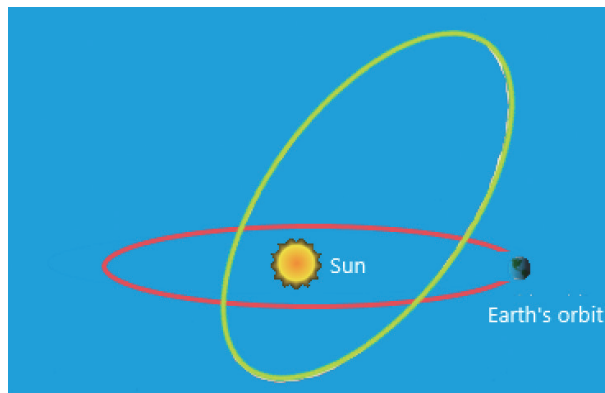
Fig. 5. The model of a meteorite stream. The red circle is Earth's orbit, and the green circle is the orbit of meteorite stream. Commonly the orbit of meteorite stream would be passed twice by Earth.
