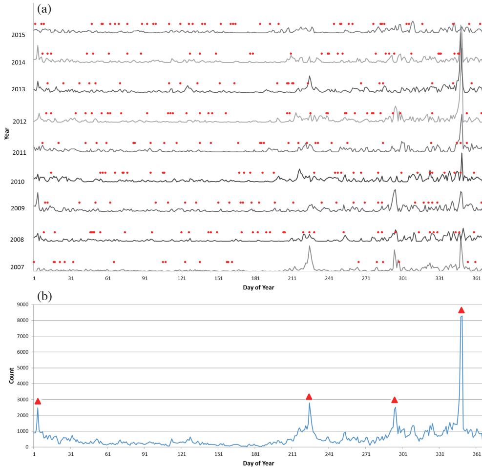
Fig. 3. (a) The bar chart of meteors with 1-day bins every year and the red round dot as fireball occurred. (b) The graph of meteors with 1-day bins. The red triangles are Quadrantids (0010 QUA), Perseids (007 PER), Draconids (009 DRA), and Geminids (004 GEM) sequentially.
