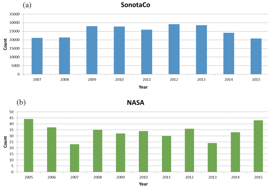
Fig. 2. (a) The bar chart for the annual rates of meteors. (b) The bar chart for the annual rates of fireballs.
